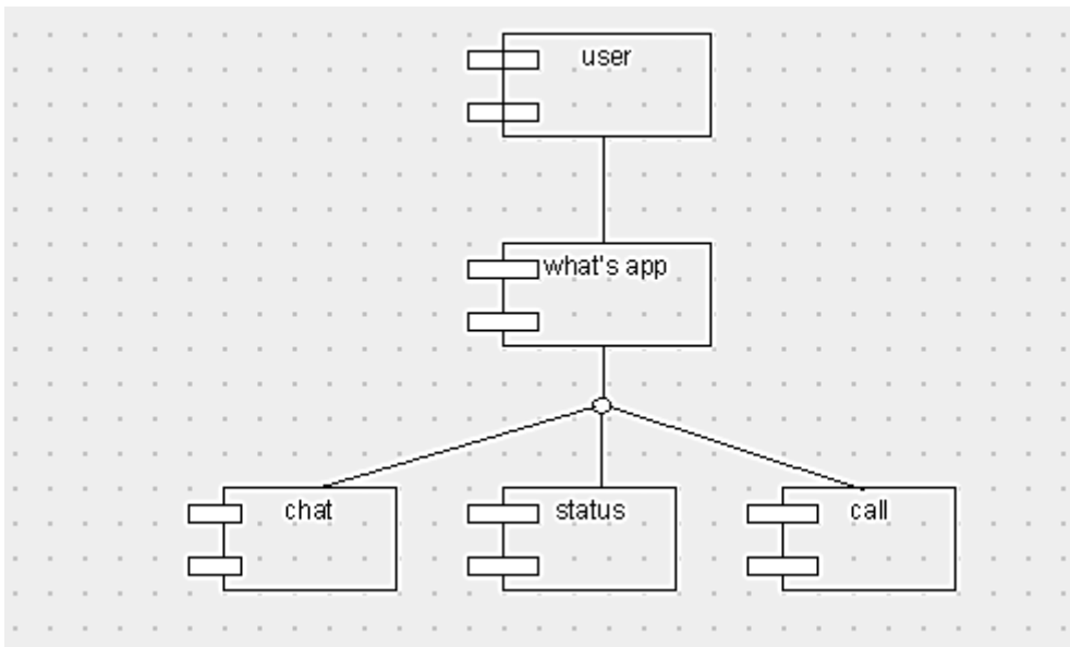
Figure 11: Component diagram
