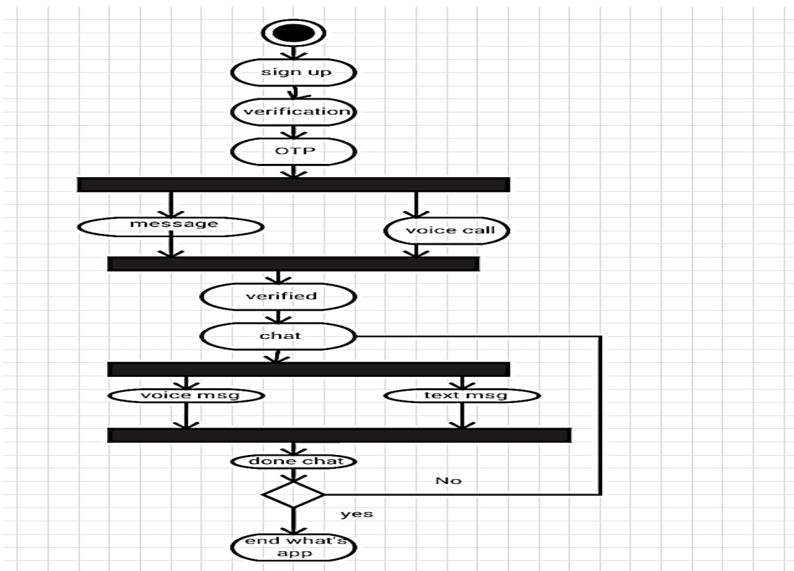
Figure 9: Activity diagram
