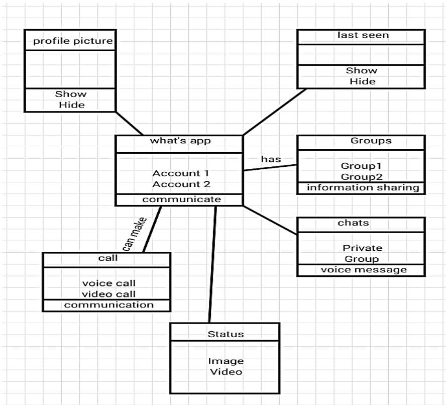
Figure 10: Class diagram
