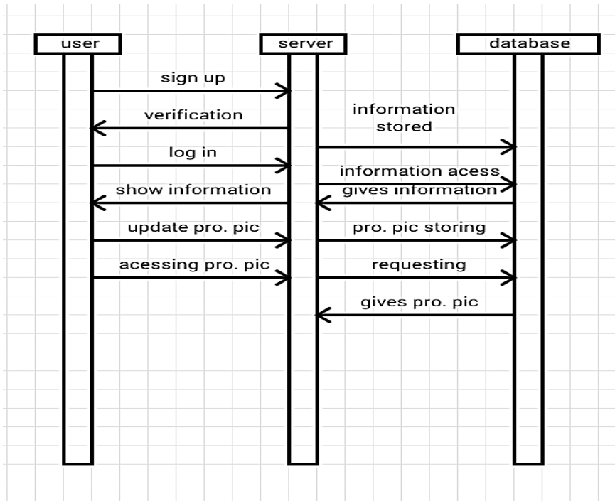
Figure 8: sequence diagram
