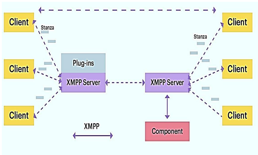
Figure 4: XMPP Architecture
